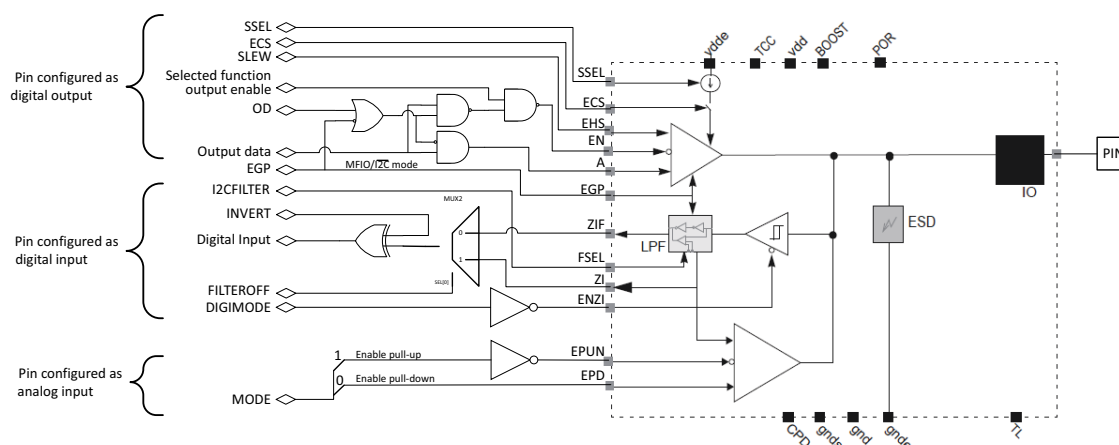
Fig 50. Combo I 2 C/GPIO pin configuration
