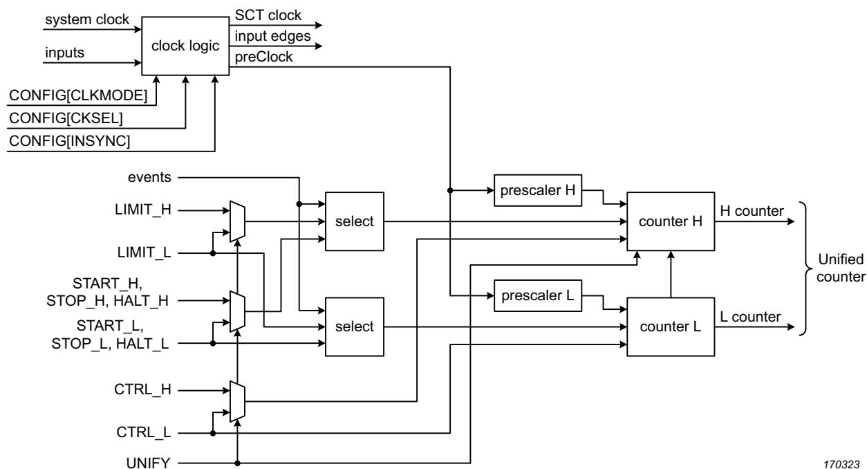
Fig 92. SCTimer/PWM counter and select logic
