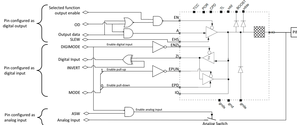
Fig 49. Standard GPIO pin configuration
