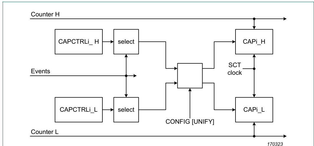
Fig 95. Capture logic
