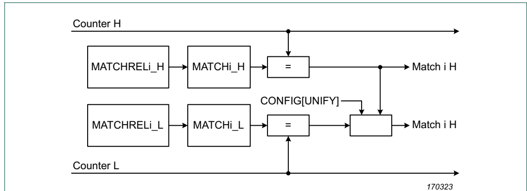
Fig 94. Match logic
