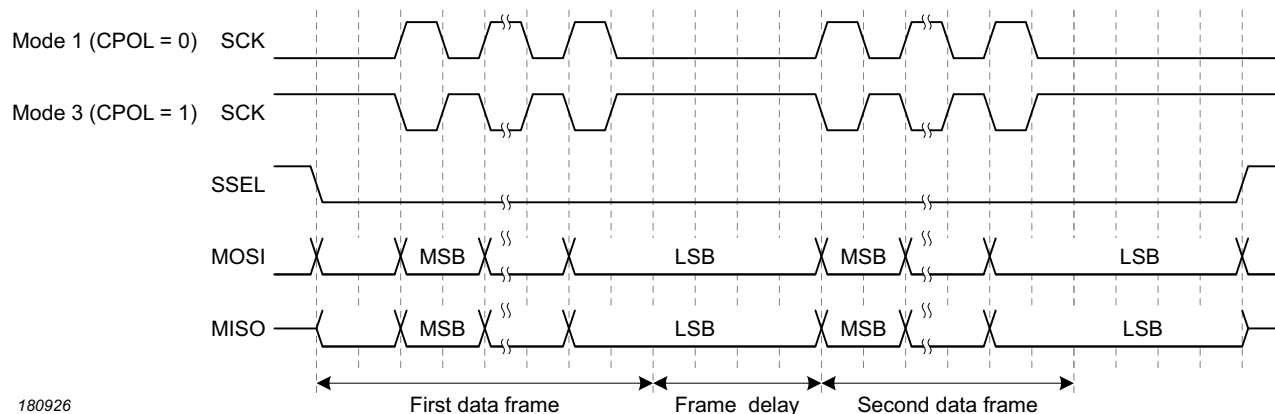
Fig 123. Frame_delay
