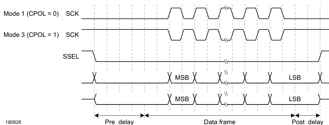
Fig 122. Pre_delay and Post_delay
