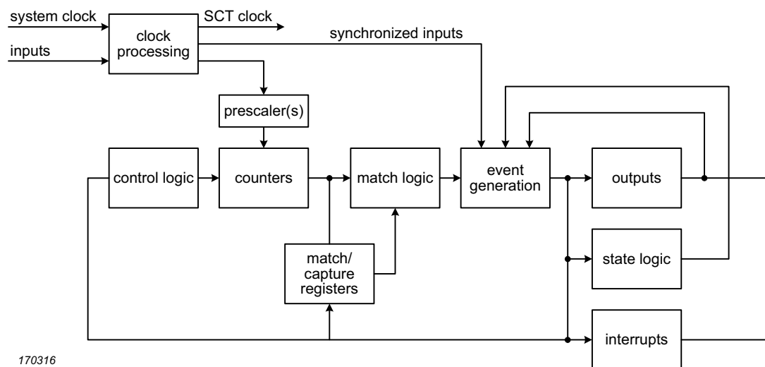
Fig 91. SCTimer/PWM block diagram
