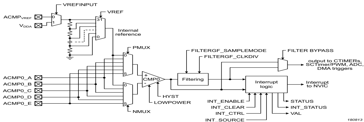
Fig 151. Comparator block diagram
