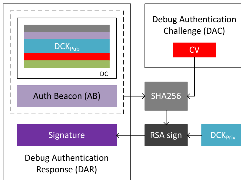
Fig 203. Debug Authentication Response (DAR) fields
