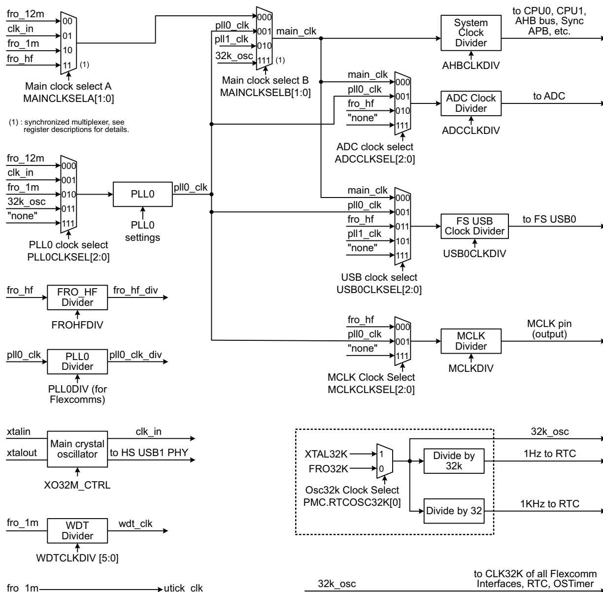
Fig 4. LPC55S6x Clock generation (Part 1 of 3)
