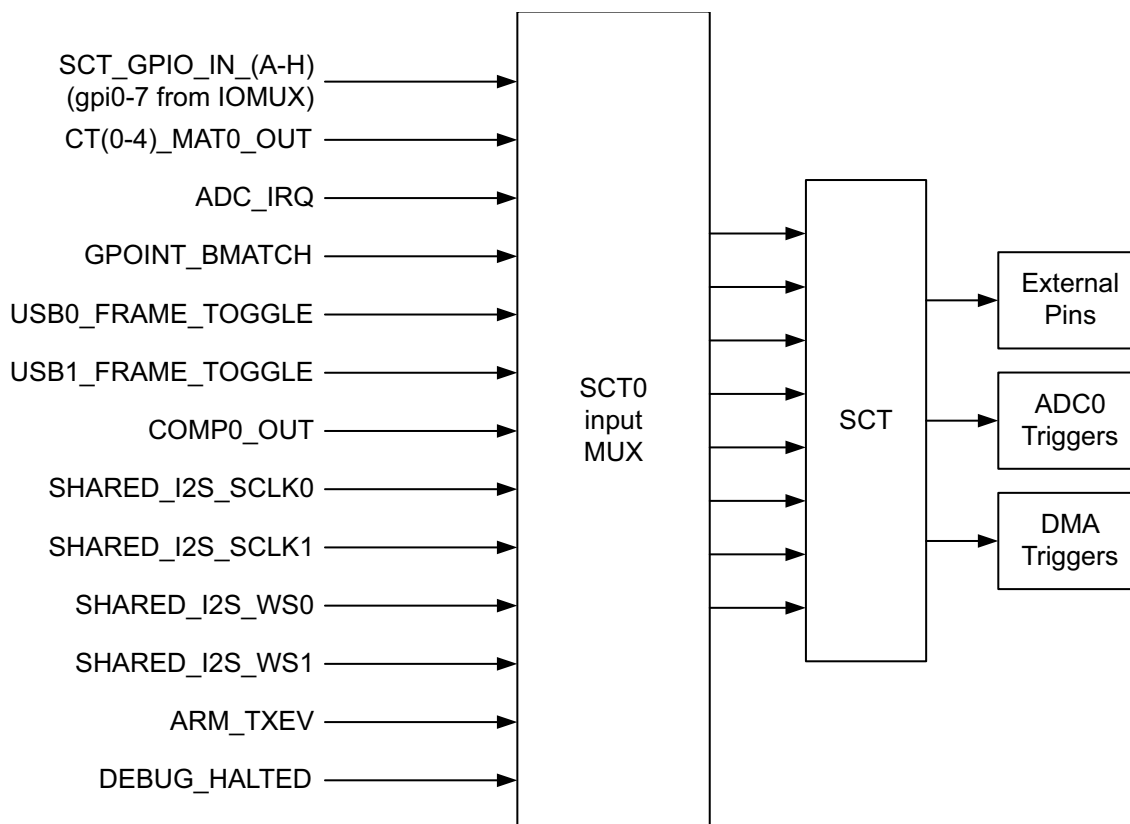
Fig 90. SCTimer/PWM connections
