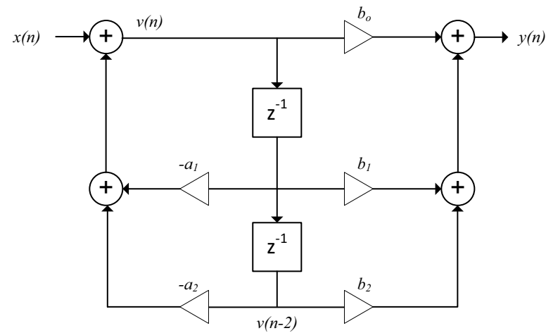
Fig 194. PowerQuad second order IIR filter
